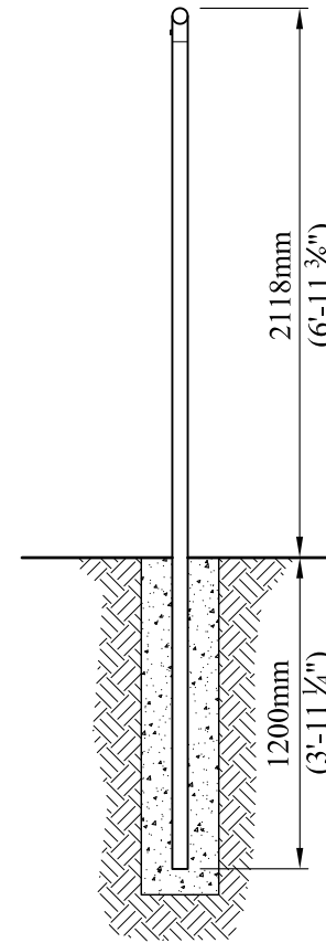
SIDE VIEW
